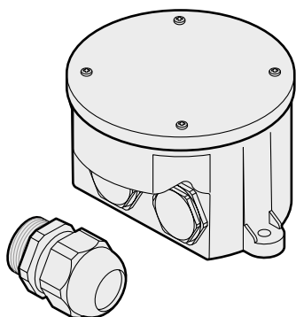
Part # AJBOX1 IP66 NEC compliant high+low voltage junction box 1/2" conduit inputs for AC + DMX, 3/4" conduit for TLAFC# Built-in AC surge protection up to 10kV & 10kA Suitable for 120-277VAC runs. Not certified for use with XTR Drivers
