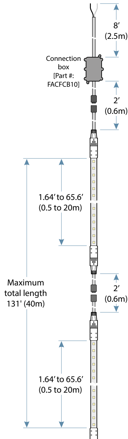
Multiple Flex 120 strips (open and terminated)
