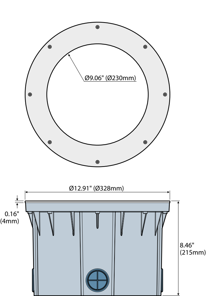
In-ground sleeve
