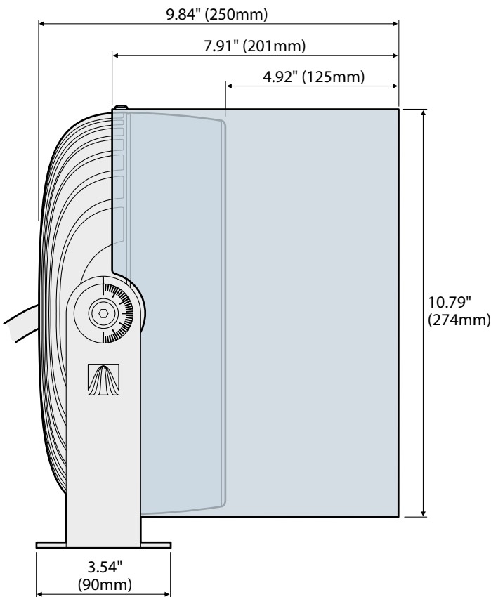
Full snoot
