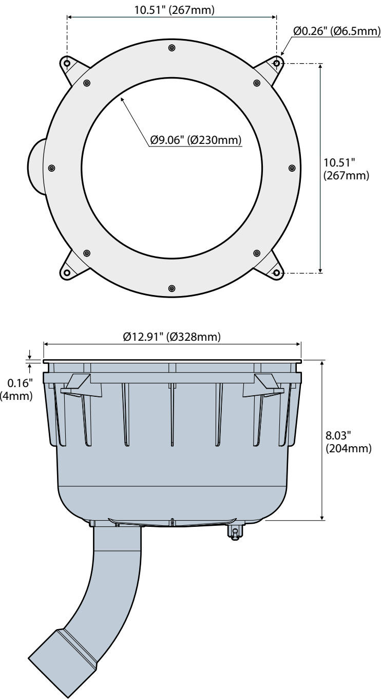
In-wall (pool niche) sleeve
