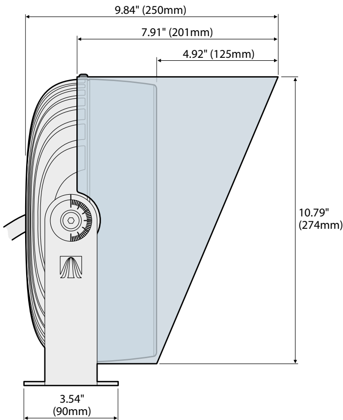
Half snoot
